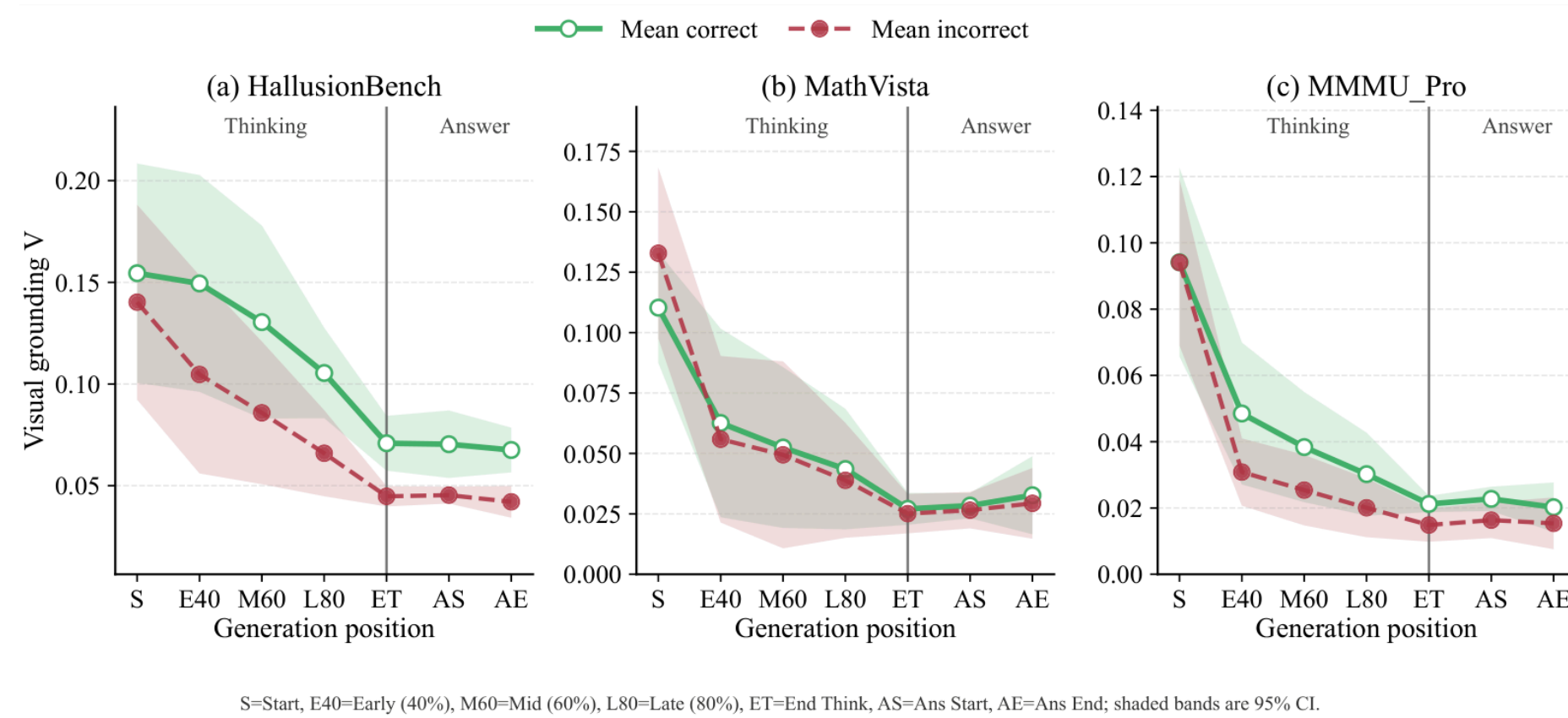
Fig. 2. Mean visual attention at seven positions; shaded bands are 95% confidence intervals. Correctness separation peaks during reasoning in 7/9 cells; MathVista shows a crossover.
