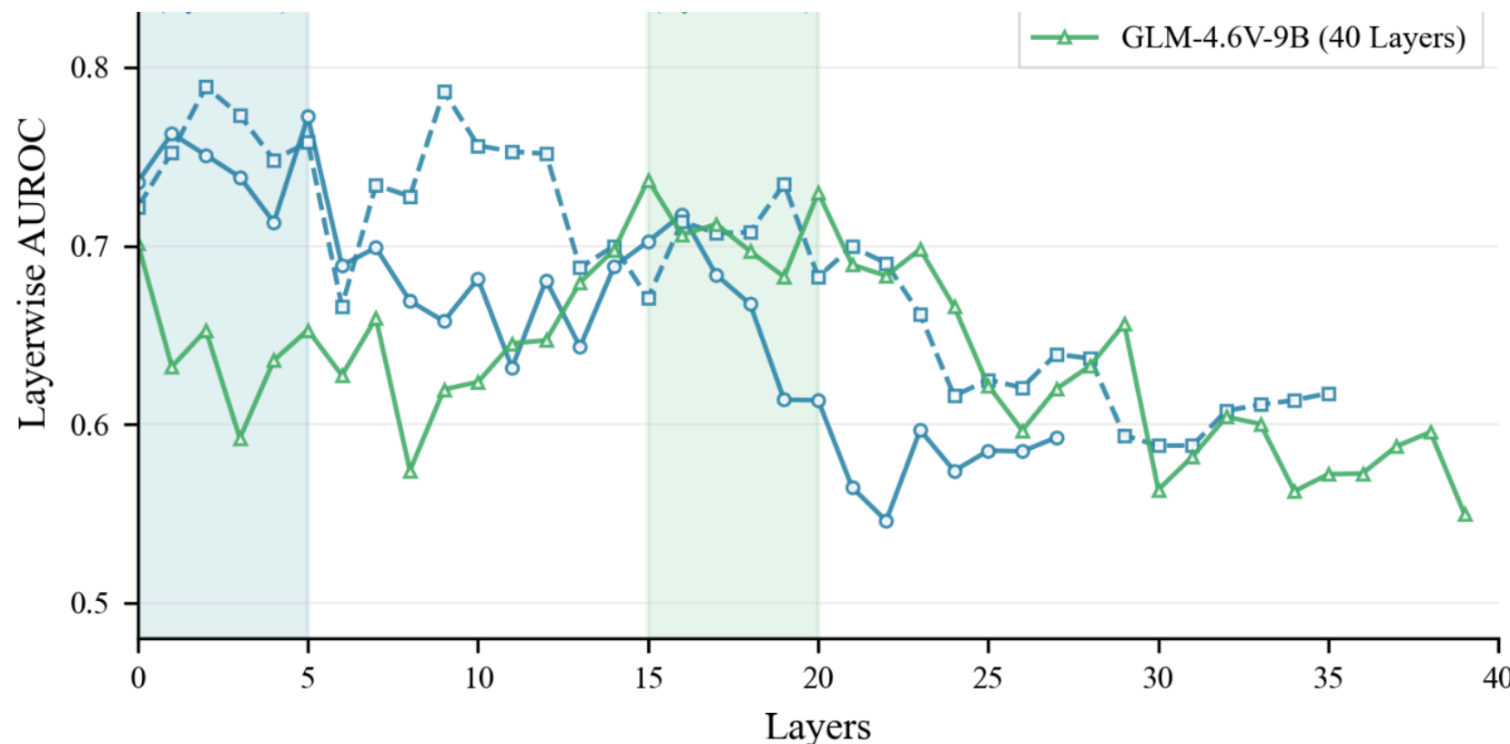
Fig. 1. Qwen3-VL-2B and 8B peak near layers 0–5; GLM-4.6V-Flash peaks near layers 15–20. Layers were selected on 100 held-out Visual-CoT samples.
