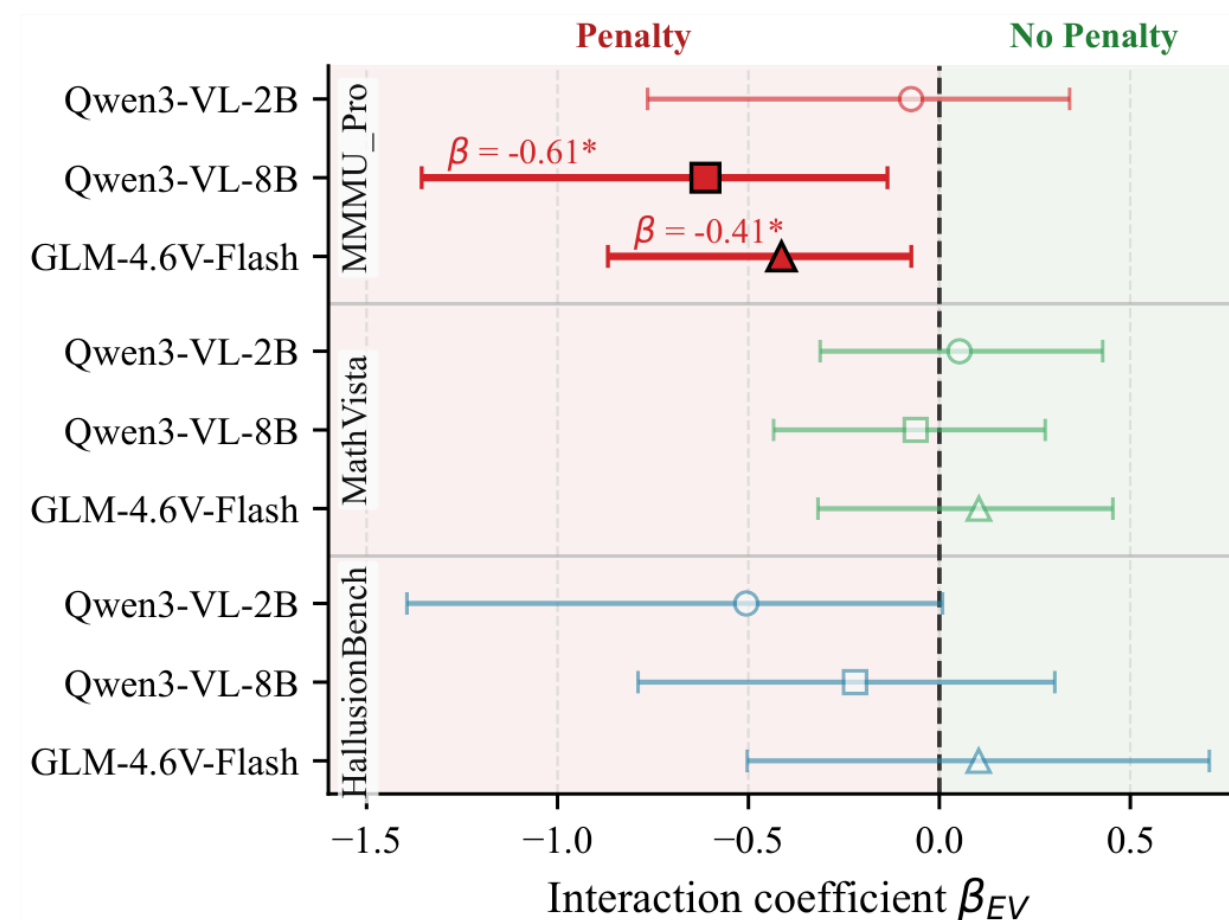
Fig. 3. Negative \beta_{EV} means low entropy plus low visual engagement predicts extra error. The penalty is significant for Qwen3-VL-8B and GLM on MMMU Pro; MathVista has no such penalty.
